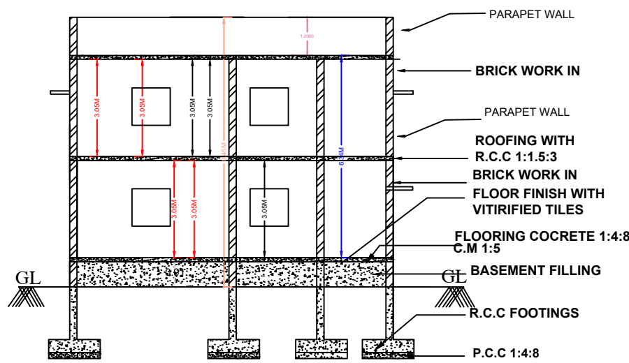
SECTION ON "BB1"
