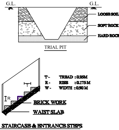
STAIRCASE & ENTRANCE STEPS
