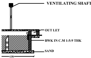
OF THE SEPTIC TANK
