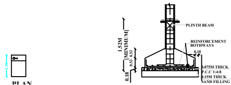
TYP.DET. COLUMN FOOTING
