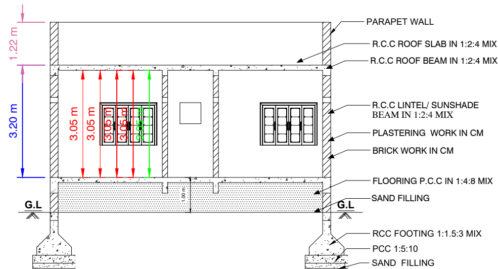
SECTION"AB"
