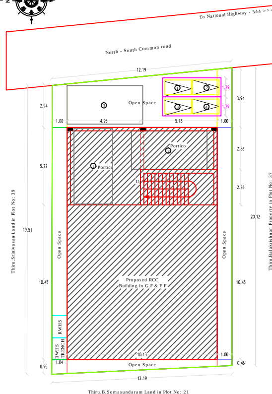
SITE PLAN - (ACTUAL AT SITE) SCALE (1:100)
