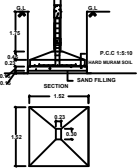
FOUNDATION DETAILS
