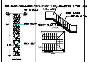
SECTIONAL DETAILS
