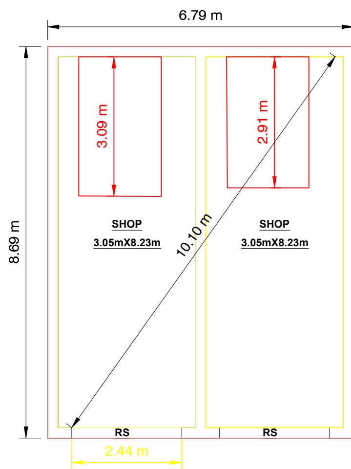
PLAN
