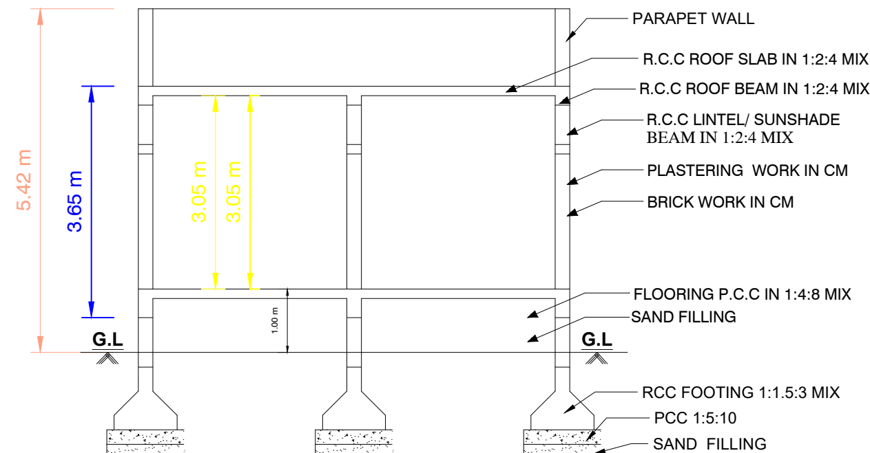
SECTION"AB"
