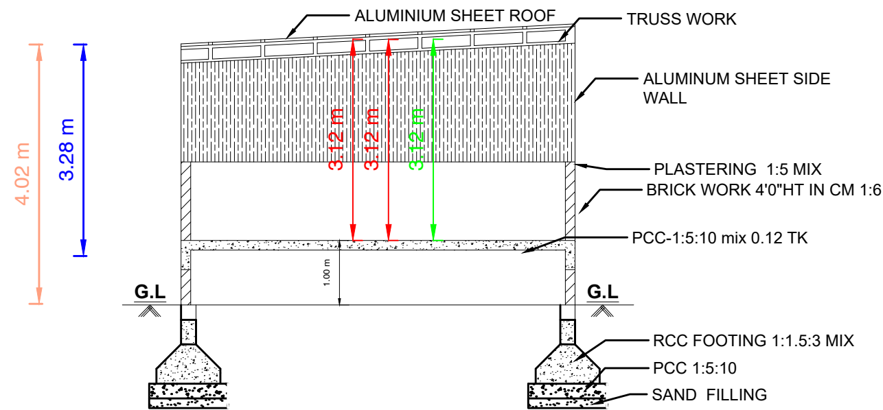
SECTION"AB"
