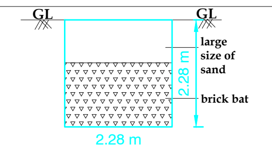
RAINWATER HARVESTING
