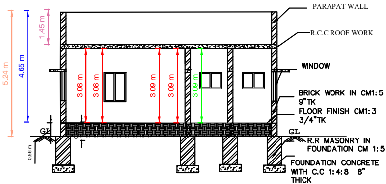
SECTION " AB "
