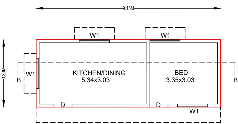
GROUND FLOOR PLAN-2 (SCALE 1:100)
