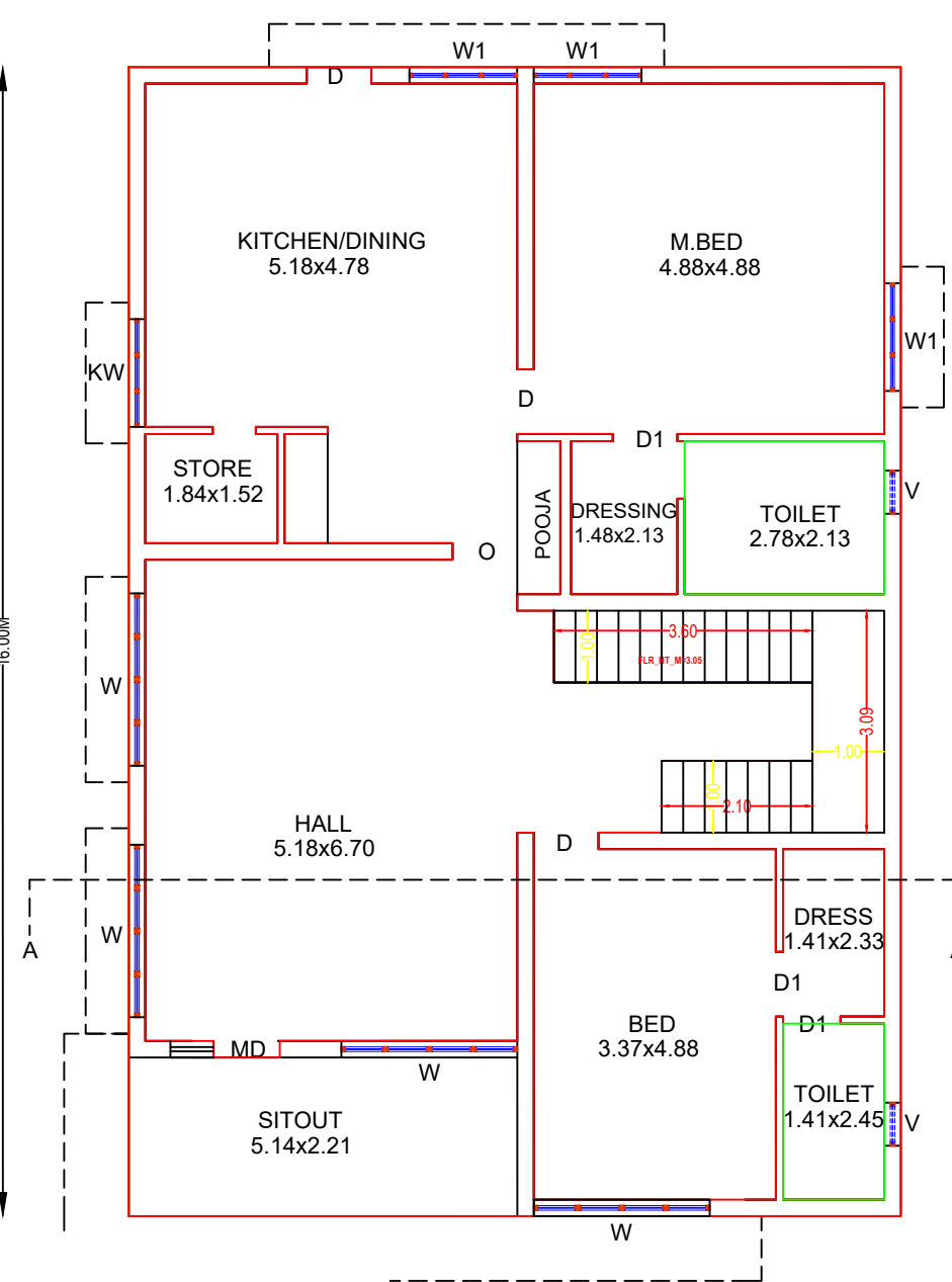
GROUND FLOOR PLAN-1 (SCALE 1:100)
