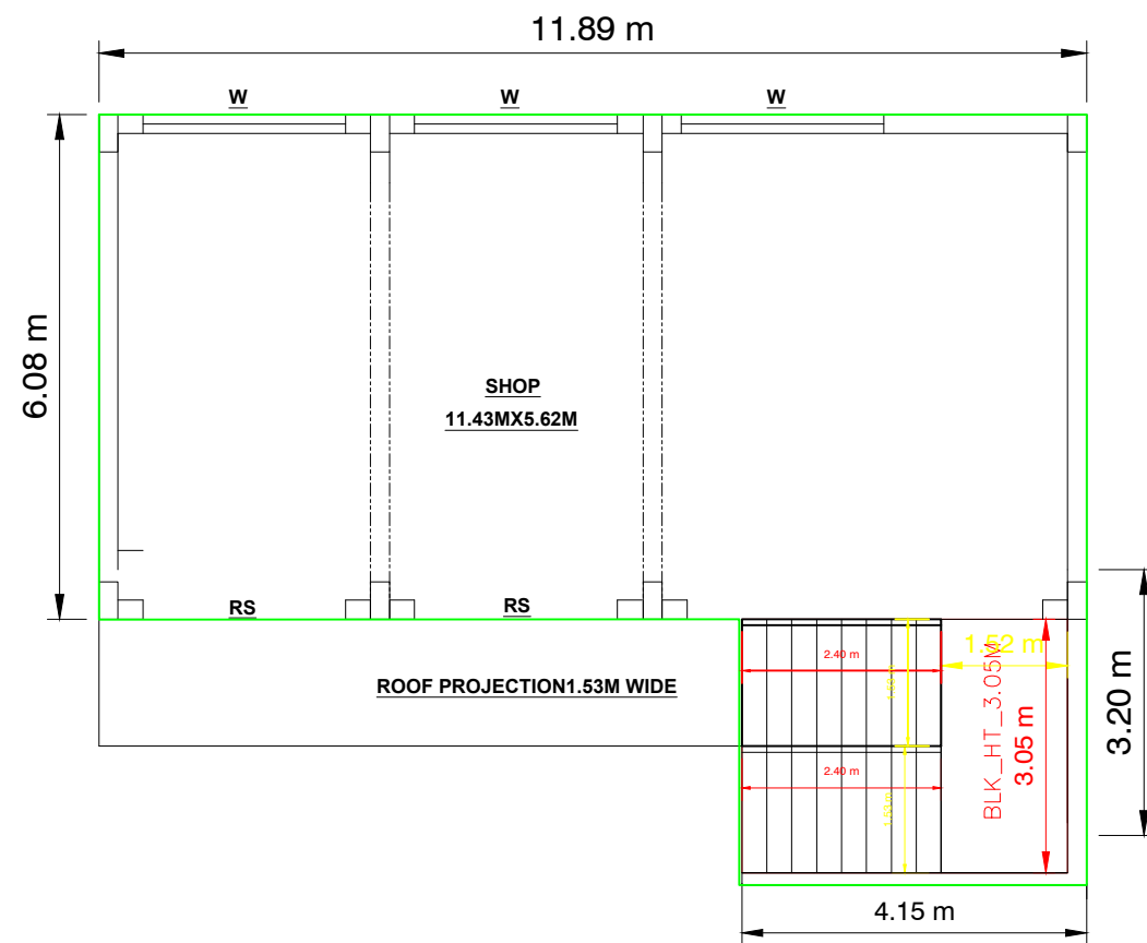
EXI-F.F PLAN
