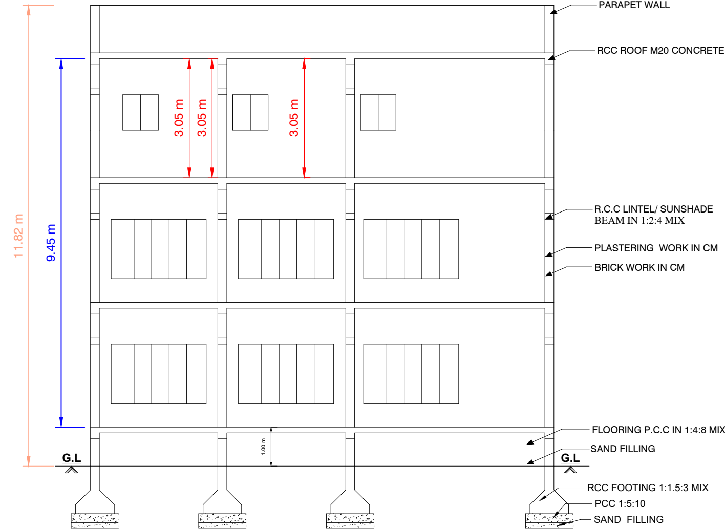
SECTION"AB"
