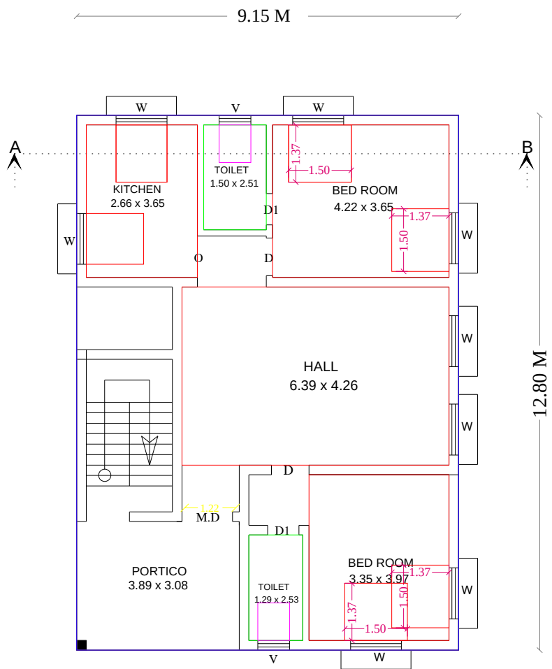
PLAN - GROUND FLOOR
