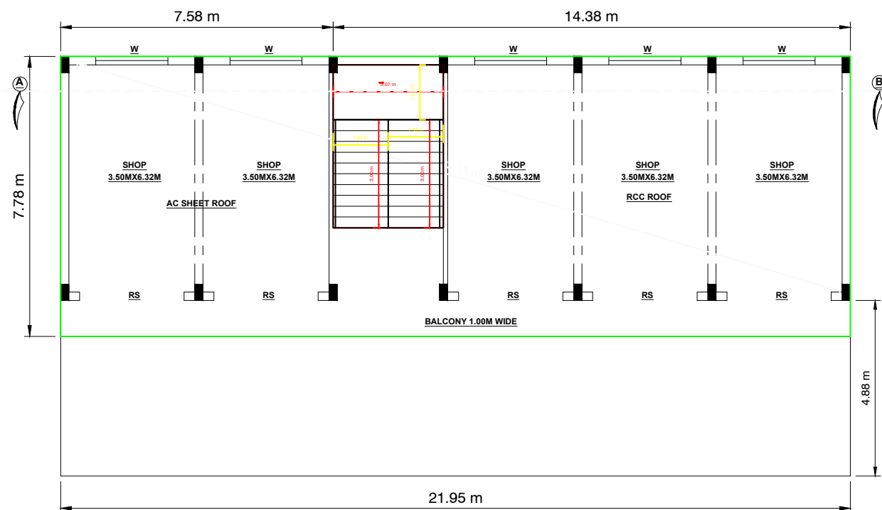
Exi-F.F PLAN
