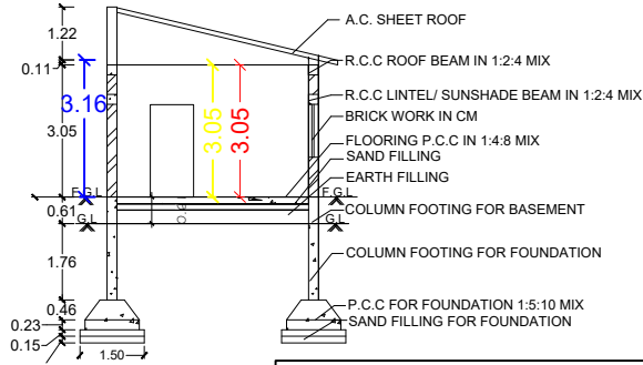
SECTION ON-AA
