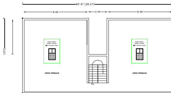
ROOF FLOOR PLAN SCALE: 1:100
