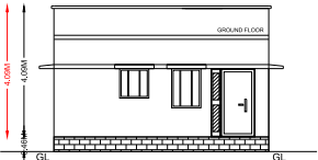
FRONT ELEVATION
