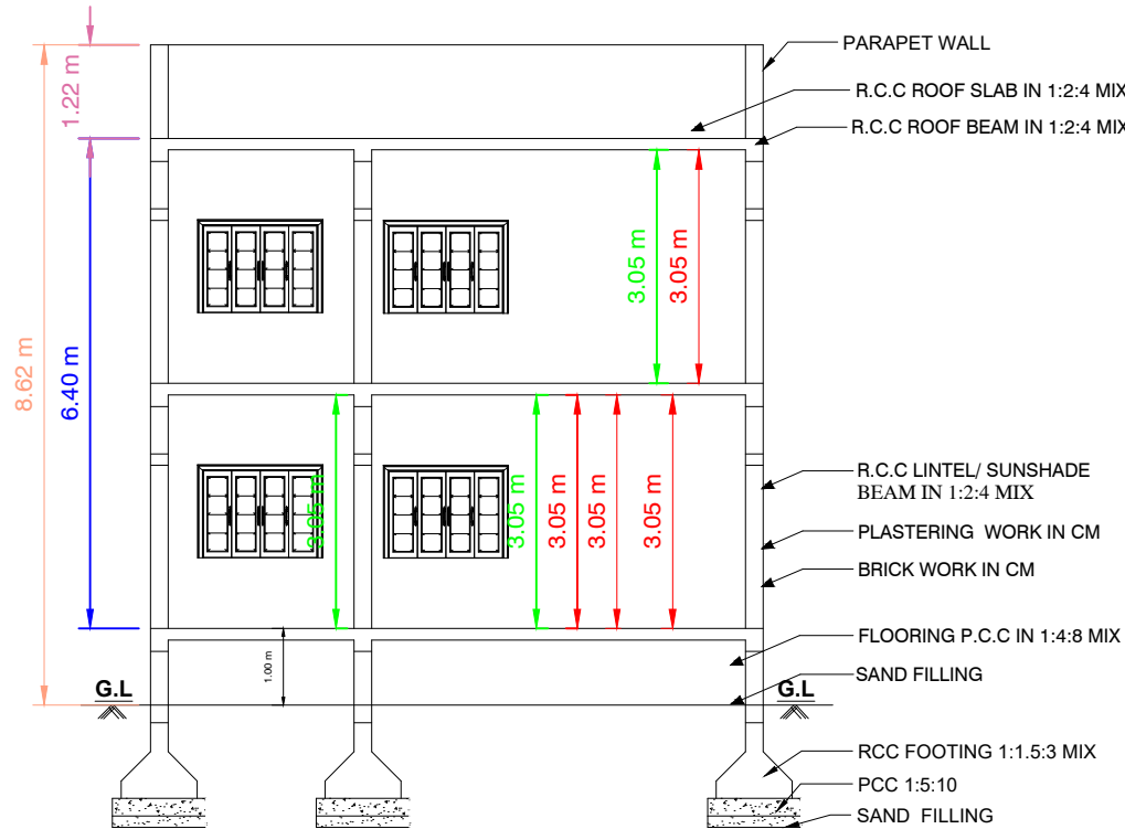
SECTION"AB"
