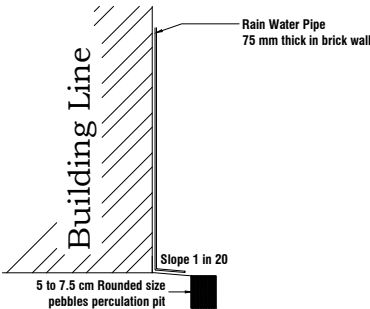
RAINWATER HARVESTING
