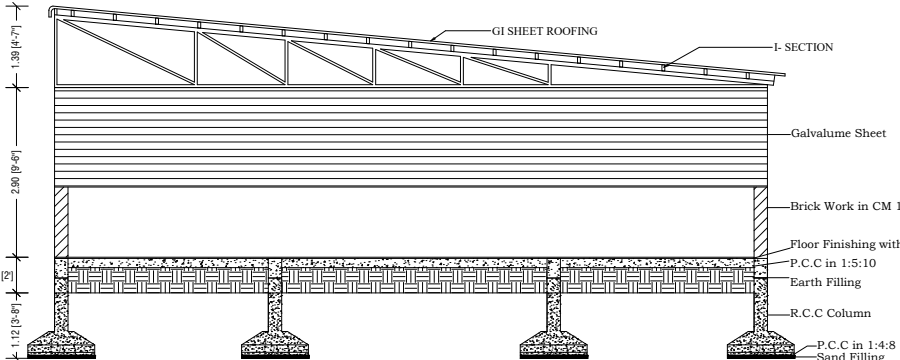
SECTION X-X
