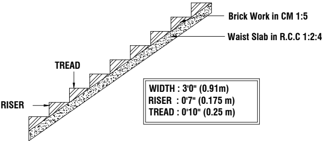
STAIRCASE DETAILS
