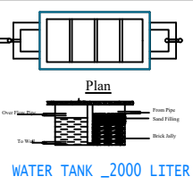
WATER TANK _2000 LITER
