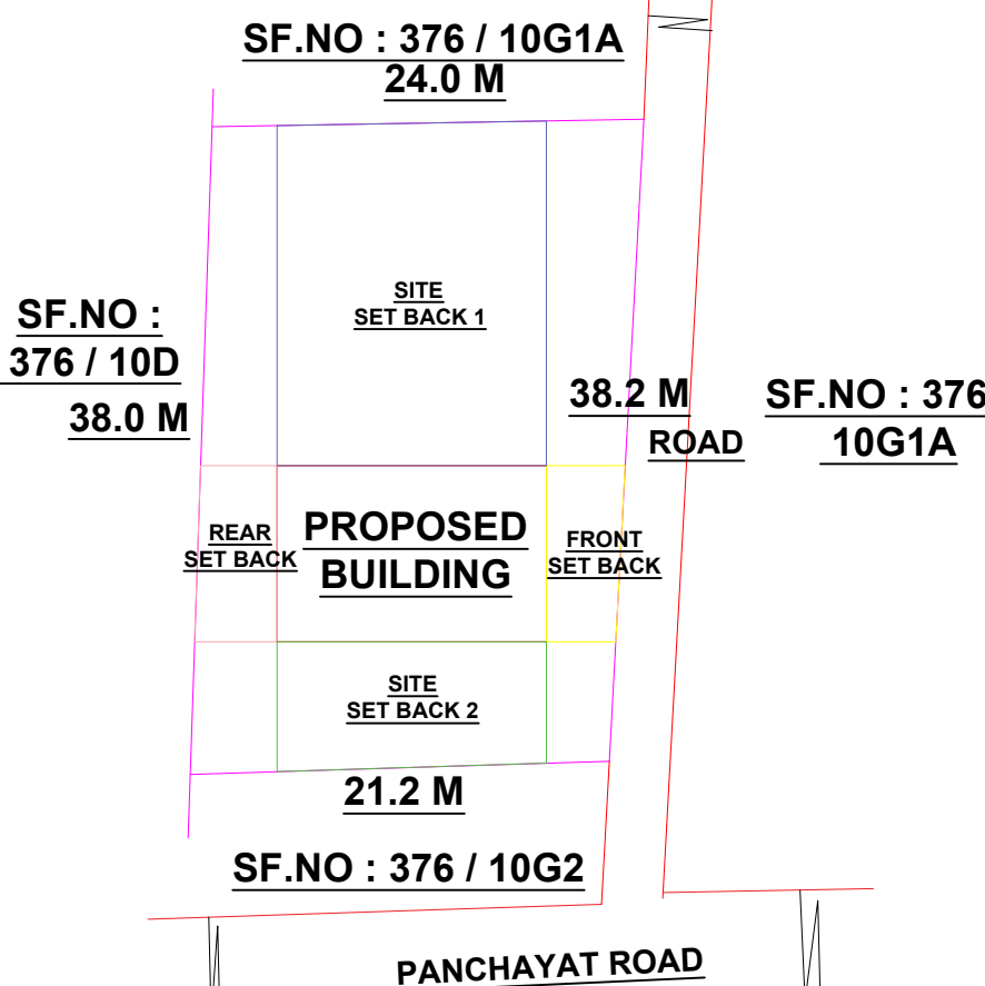
TOPO PLAN :-
