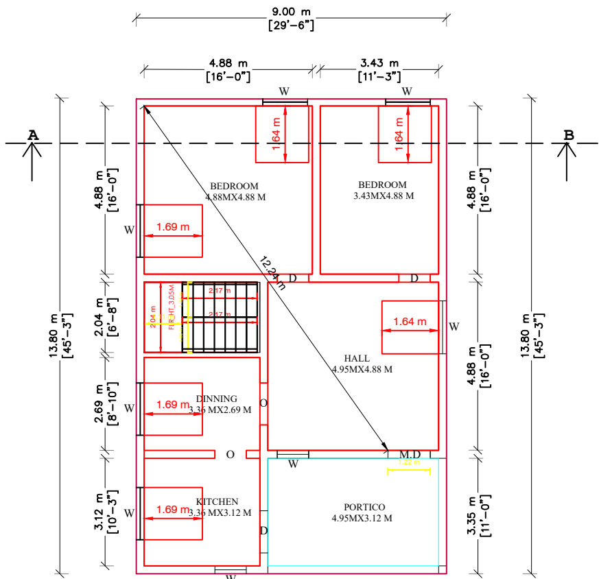
PLAN SCALE ( 1:100 )
