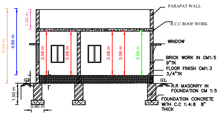
SECTION " AB "
