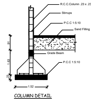
COLUMN DETAIL
