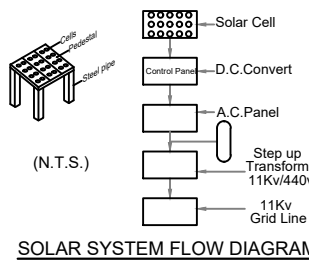
SOLAR SYSTEM FLOW DIAGRAM
