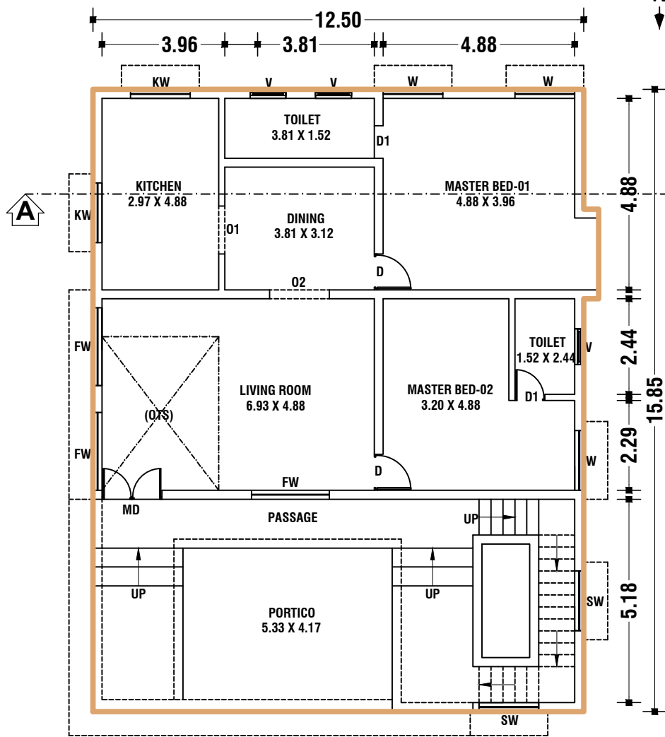
NORTH FACING GROUND FLOOR PLAN APPROVED -EXISTING BUILDING
