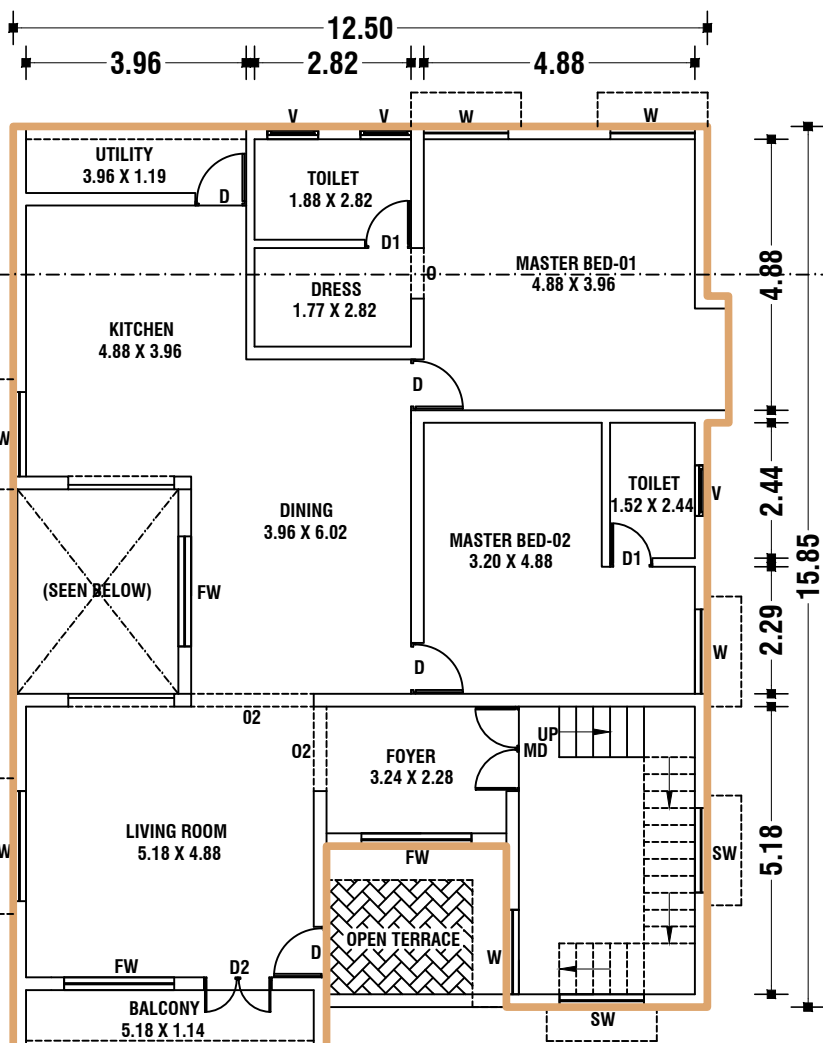
NORTH FACING FIRST FLOOR PLAN APPROVED -EXISTING BUILDING
