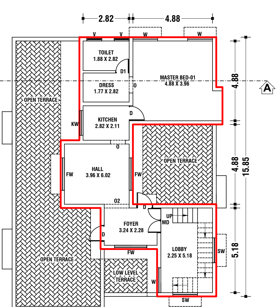
NORTH FACING SECOND FLOOR PLAN ADDITIONAL PROPOSED BUILDING
