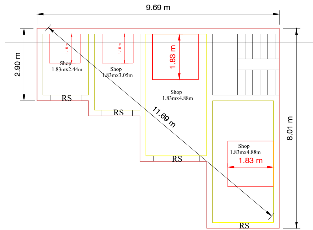
COMMERCIAL - PLAN
