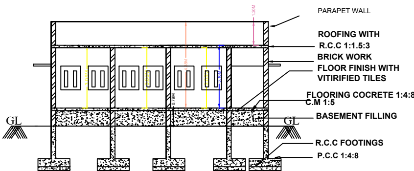
SECTION ON "BB1"
