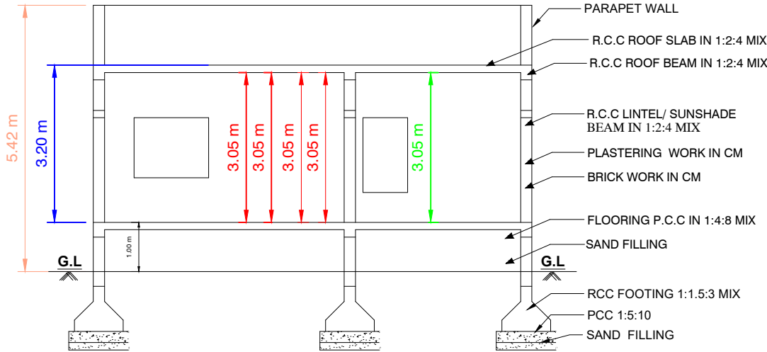
SECTION"AB"
