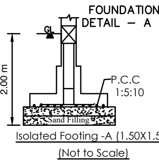
Foundation Detail - A (Not to Scale)
