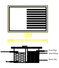
WATER TANK ,2000 LITER
