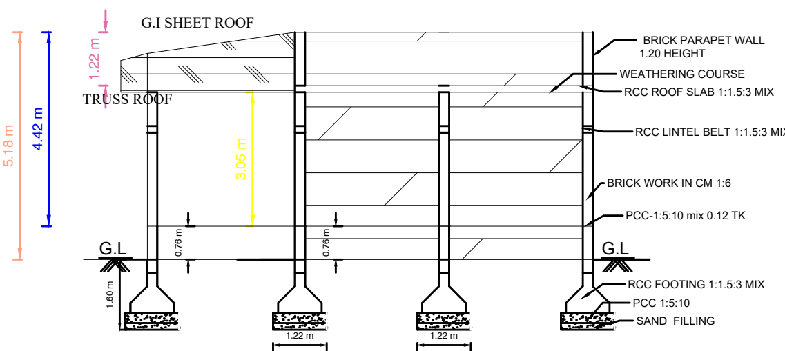
SECTION " AB "
