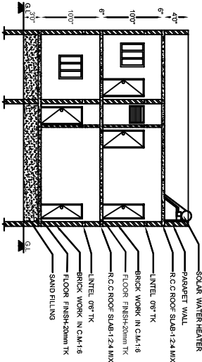
CROSS SECTION ON (A-B)
