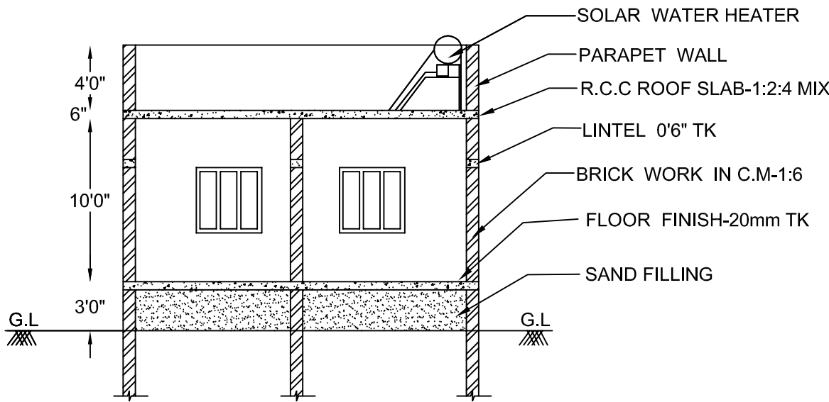
CROSS SECTION ON - 'AB'
