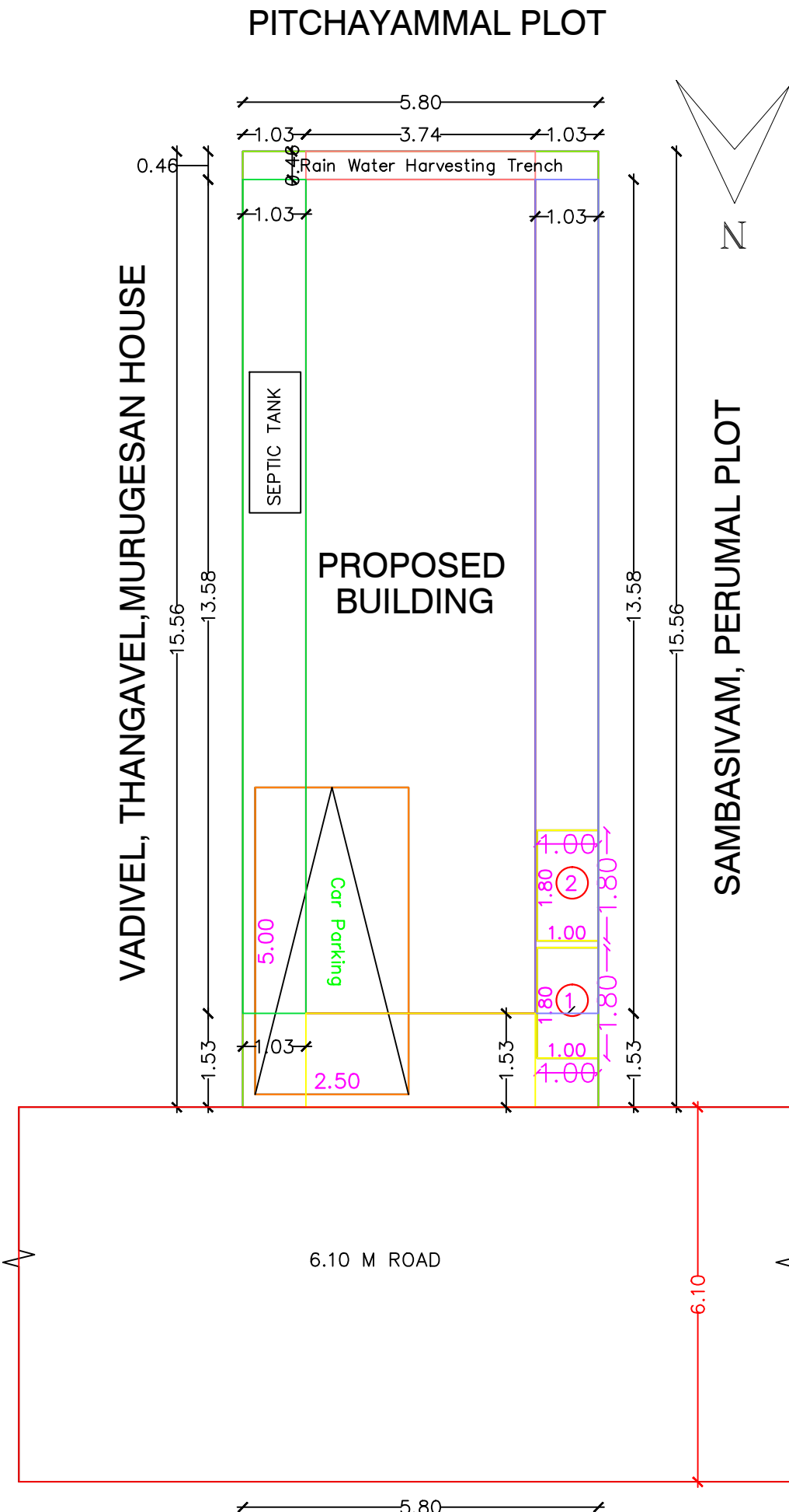
SITE PLAN
