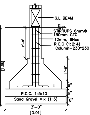
R.C.C. COLUMN FOOTING DETAILS SCALE : 1:25
