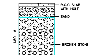
RAIN WATER HARVEST COLLECTION PIT.
