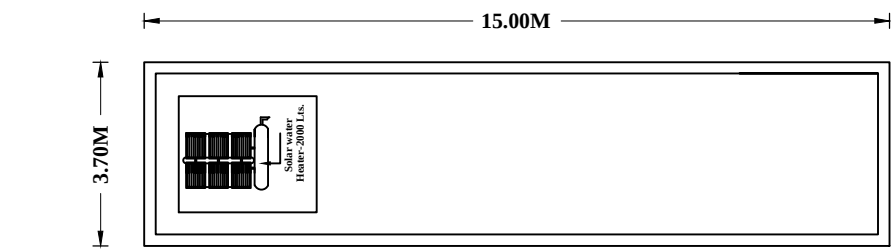
TERRACE FLOOR PLAN
