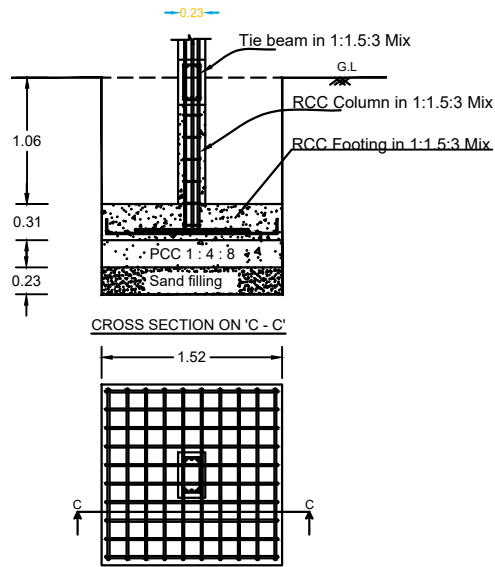
COLOUMN FOUNDATION
