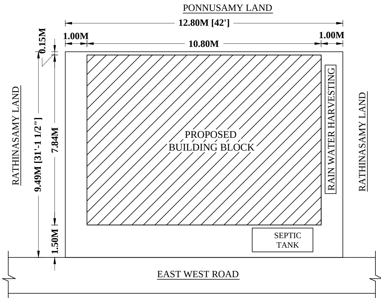
SITE PLAN SCALE IN -1:100
