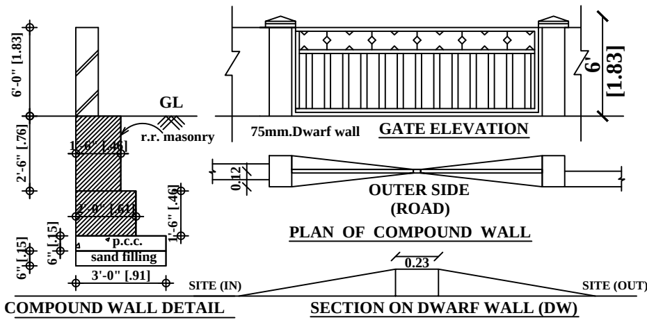
SECTION ON DWARF WALL (DW)
