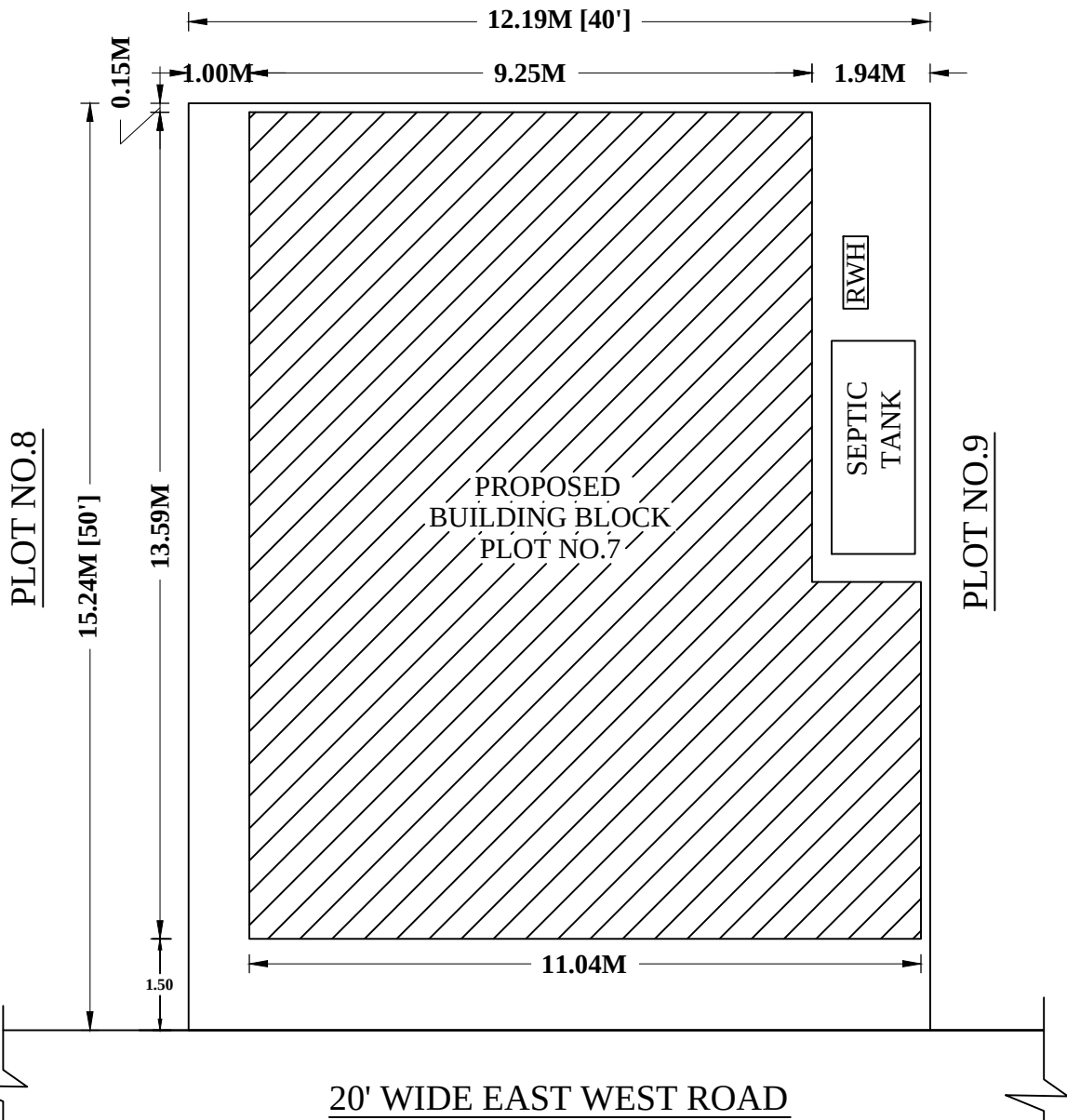
SITE PLAN SCALE IN -1:100
