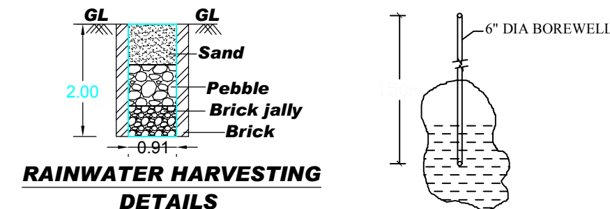
BORE WELL DETAILS
