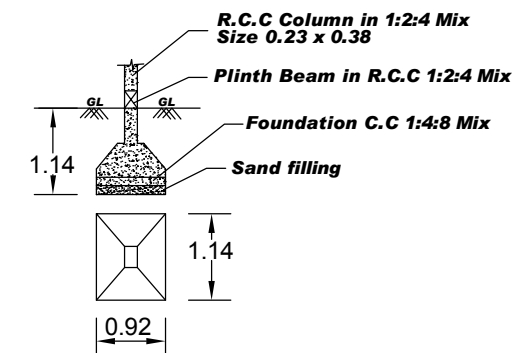
COLUMN DETAILS
