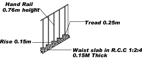
STAIRCASE SECTION
