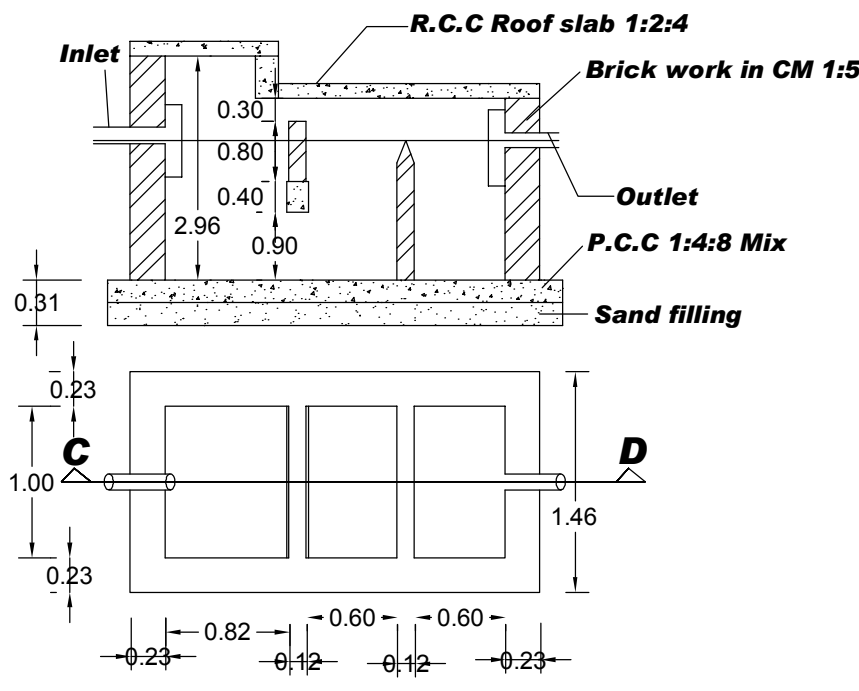
SEPTIC TANK DETAILS [SCALE 1:50]
