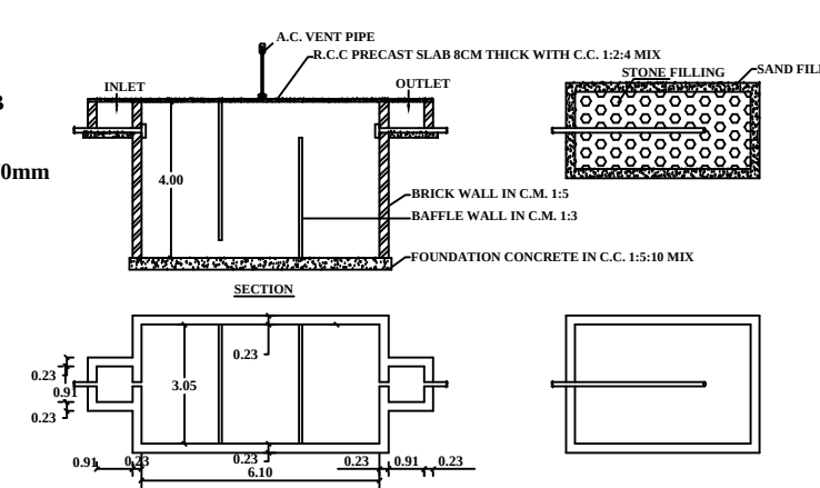
PLAN PLAN & SECTION OF SEPTIC TANK & DISPERSION TRENCH
