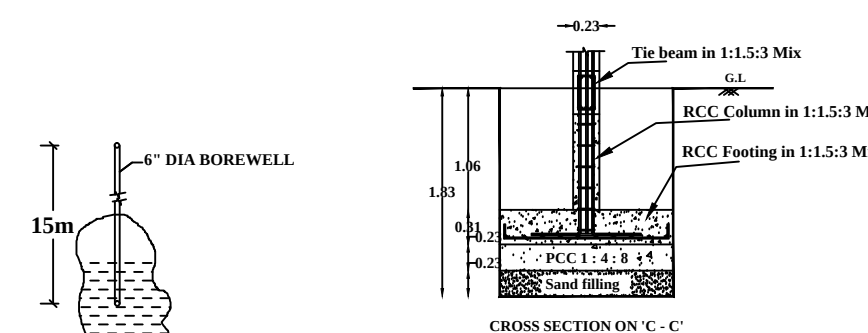
COLOUMN FOUNDATION DETAILS
