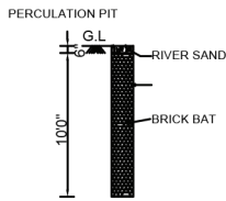
PERCOLATION PIT
