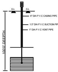
BORE WELL
