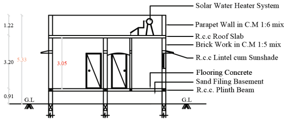
SECTION ON-"AA"
