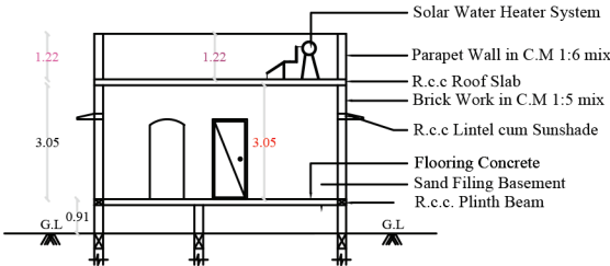
SECTION ON-"AA"
