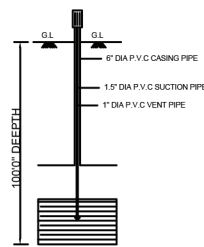
BORE WELL
