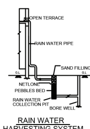
RAIN WATER HARVESTING SYSTEM
