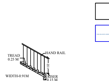
STAIRCASE DETAILS
