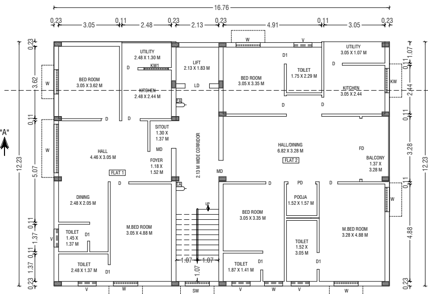
TYPICAL (FIRST, SECOND, THIRD, FOURTH & FIFTH) FLOORS PLAN
