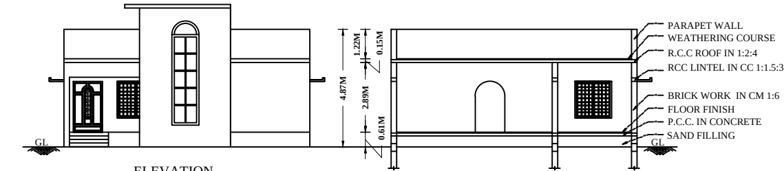
SECTION ON AB
