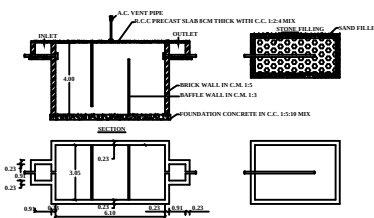
PLAN & SECTION OF SEPTIC TANK & DISPERSION TRENCH
