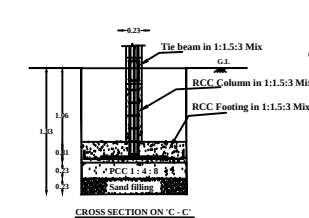
COLOUMN FOUNDATION DETAILS
