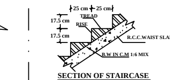
SECTION OF STAIRCASE
