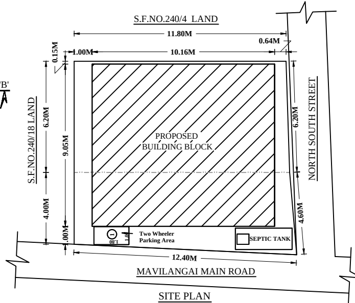
SITE PLAN SCALE IN -1:100
