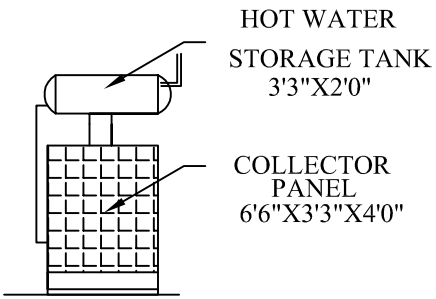
FRONT ELEVATION SOLAR WATER HEATER
