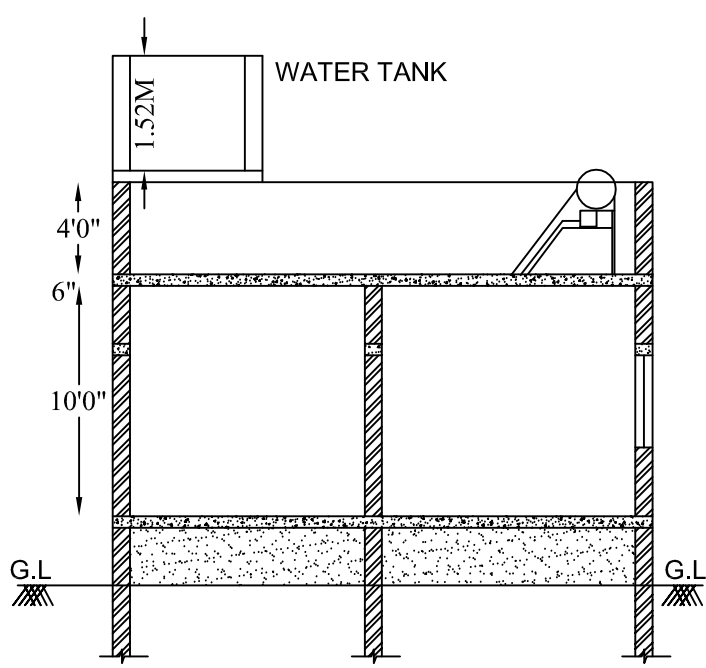
CROSS SECTION (A-B)
