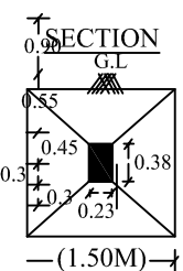
DETAILS OF COLUMN FOUNDATION
