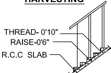
STAIRCASE DETAILS
