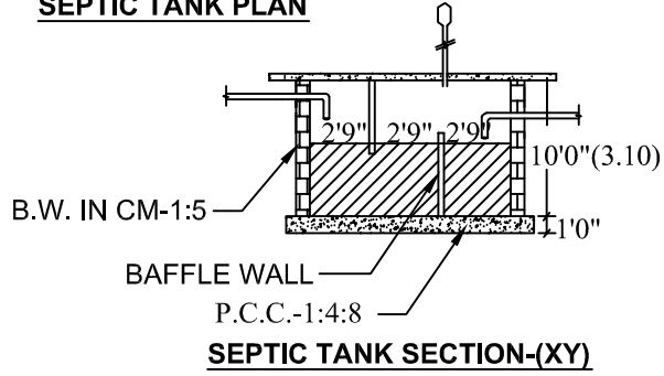
SEPTIC TANK SECTION-(XY)
