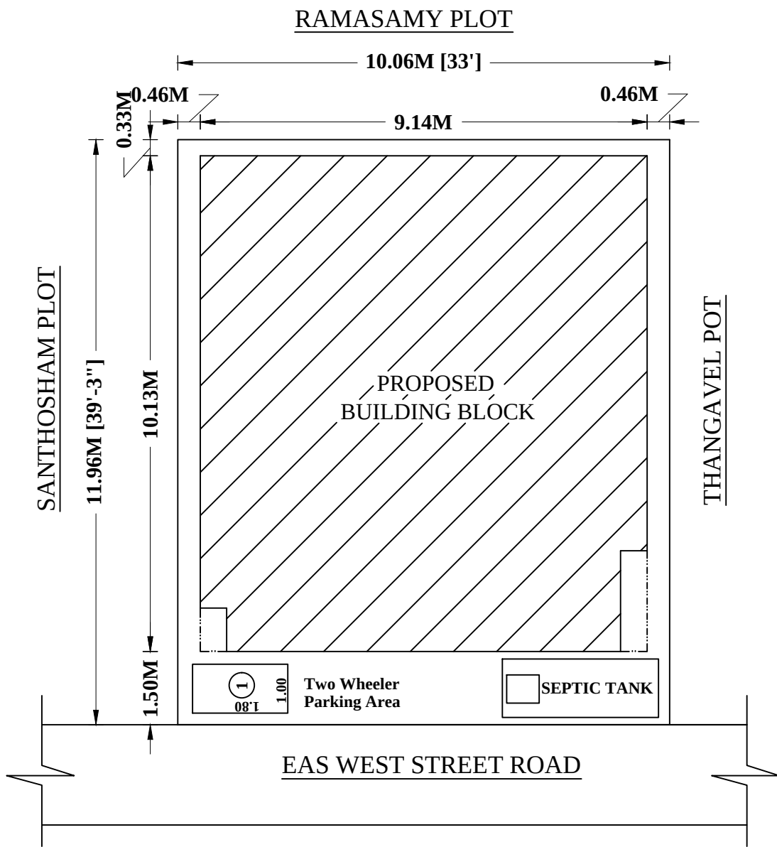
SITE PLAN SCALE IN -1:100
