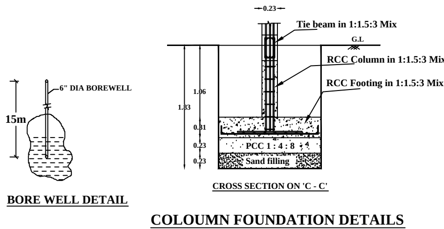
COLOUMN FOUNDATION DETAILS
