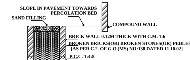
SECTION OF RAIN WATER PERCOLATION BED
