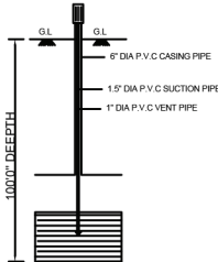
BORE WELL
