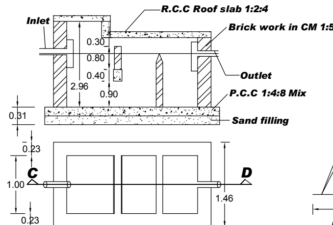
SEPTIC TANK DETAILS [SCALE 1:50]
