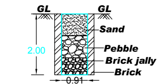
RAINWATER HARVESTING DETAILS
