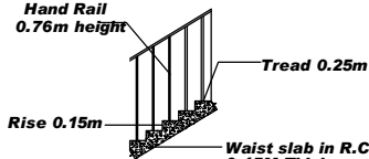
STAIRCASE SECTION
