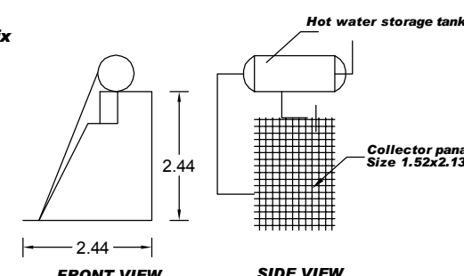
SOLAR WATER HEATER DETAILS [SCALE 1:100]
