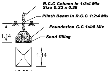
COLUMN DETAILS
