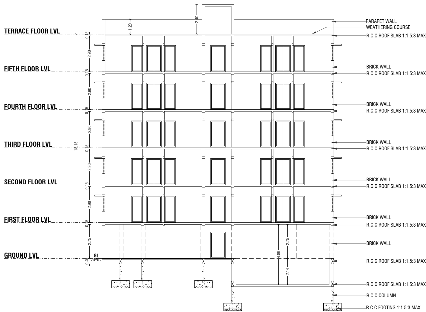
SECTION PLAN @ NORTH SIDE
