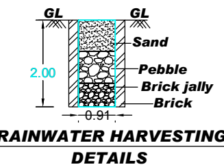
RAINWATER HARVESTING DETAILS
