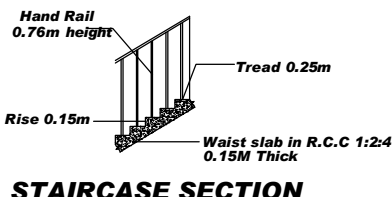
STAIRCASE SECTION
