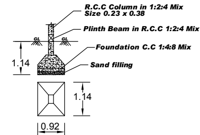
COLUMN DETAILS
