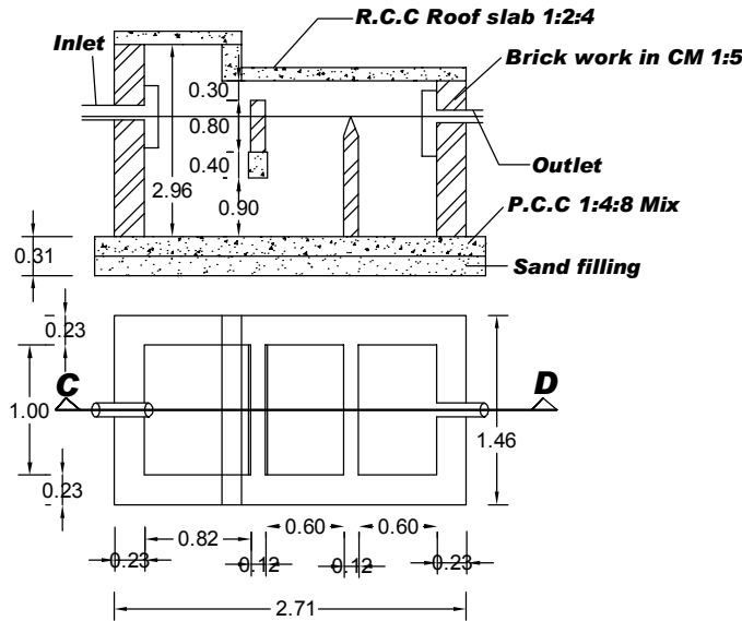
SEPTIC TANK DETAILS [SCALE 1:50]
