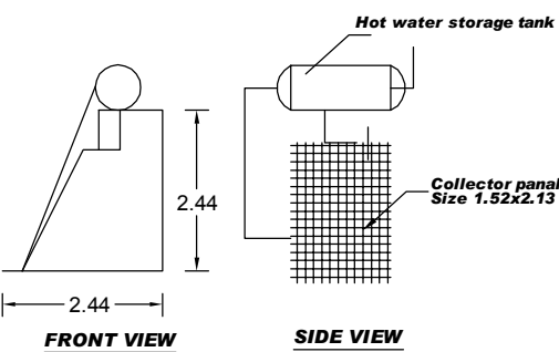
SOLAR WATER HEATER DETAILS [SCALE 1:100]
