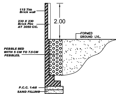
SECTION OF COMPOUND WALL & RAINWATER COLLECTING PIT
