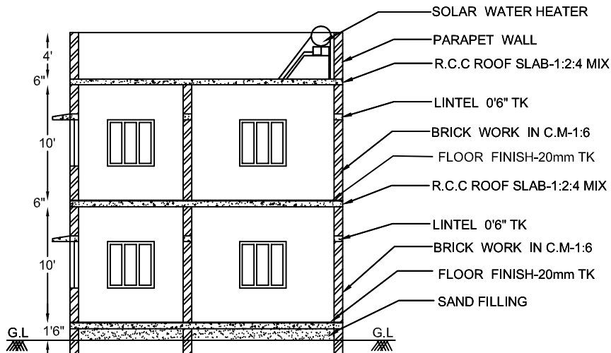
CROSS SECTION ON (A-B)
