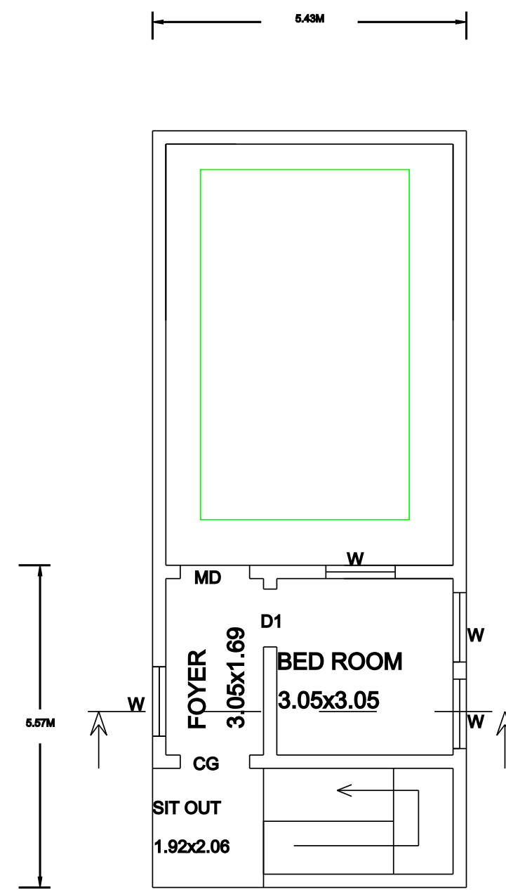
FIRST FLOOR
