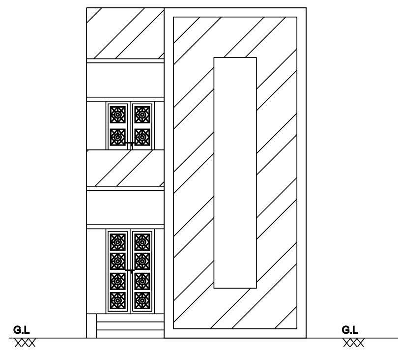
FRONT ELEVATION
